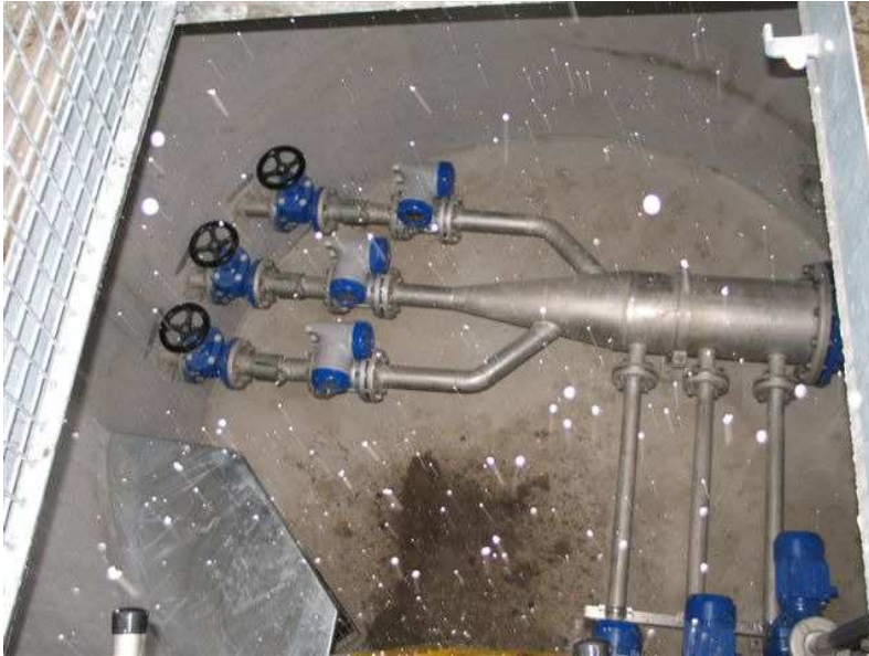
14.11.2007 – Flow meter structure, outlet from filters
